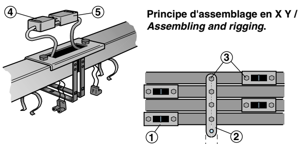
Ensemble "SOLO 744 A" (6 pièces) / "SOLO 744 A" SET (6 units).
