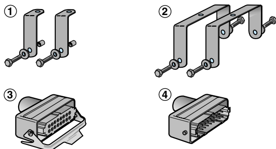
Accessoires et rechange / Spare parts and accessories.
