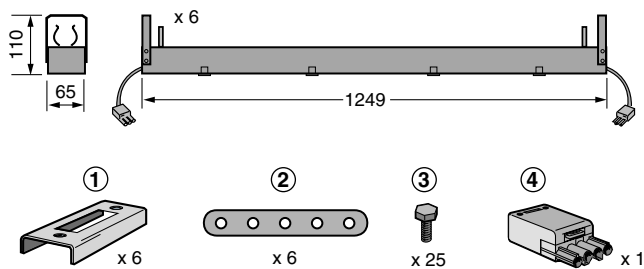
Ensemble "SOLO 744 A" (6 pièces) / "SOLO 744 A" SET (6 units).
