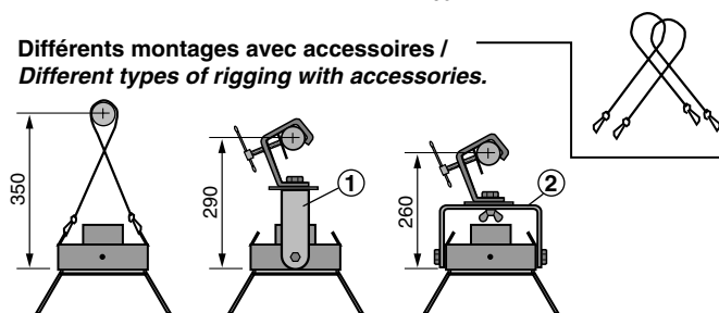
Accessoires et rechange / Spare parts and accessories.
